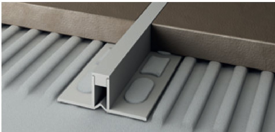
NJ/10 PVC co-extruded PVC light grey RAL 7035
